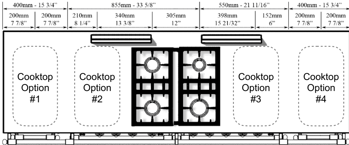
[2205mm] Sully 2200 4 Burner:
