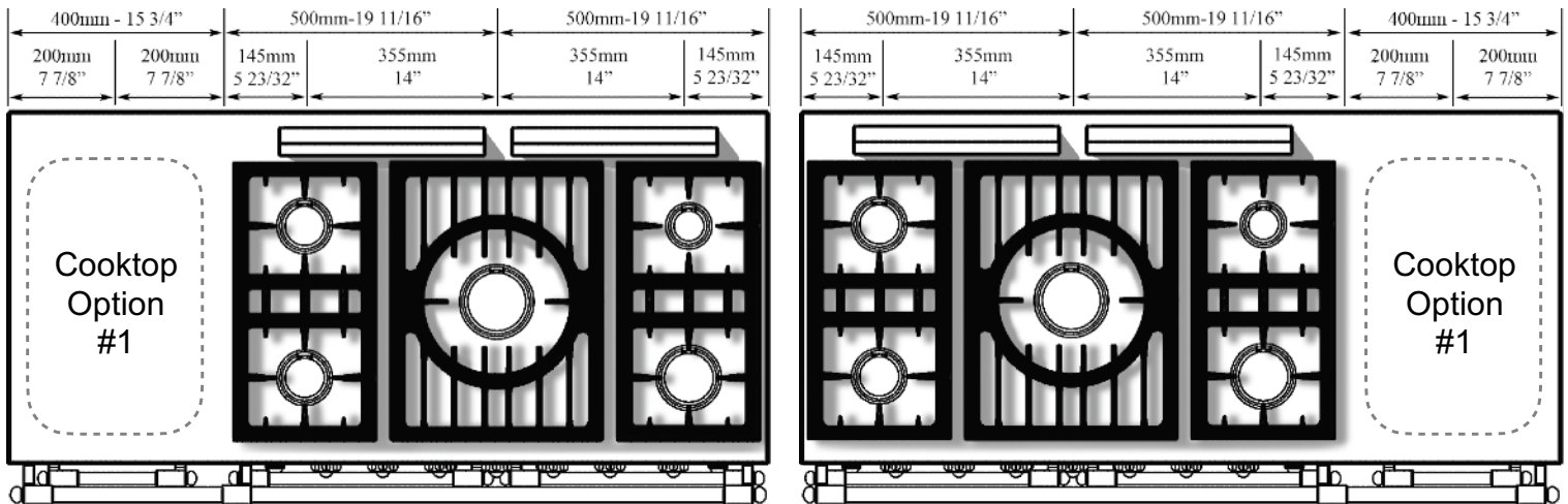
[1405mm] Sully 1400 3 & 4 Burner:
