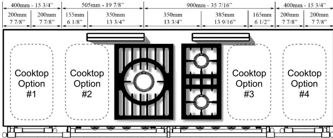
[2205mm] Sully 2200 3 Burner:
