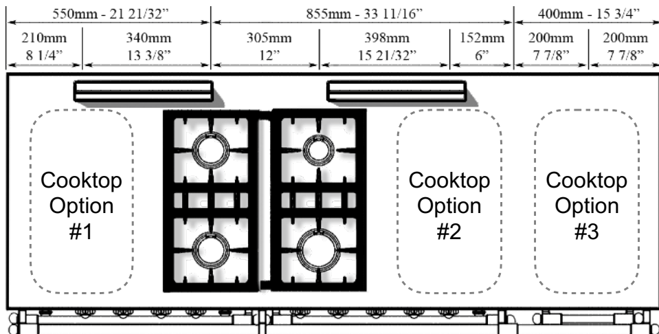
[1805mm] Sully 1800-D 4 Burner:
