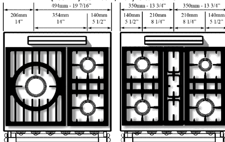
[700mm] Cormatin / Rully 3 & 4 Burner:
