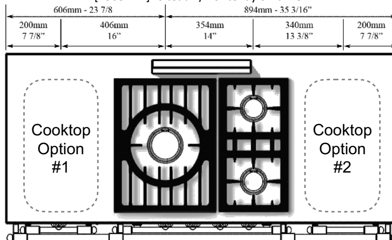
[1505mm] Citeaux / Fontenay 3 Burner:
