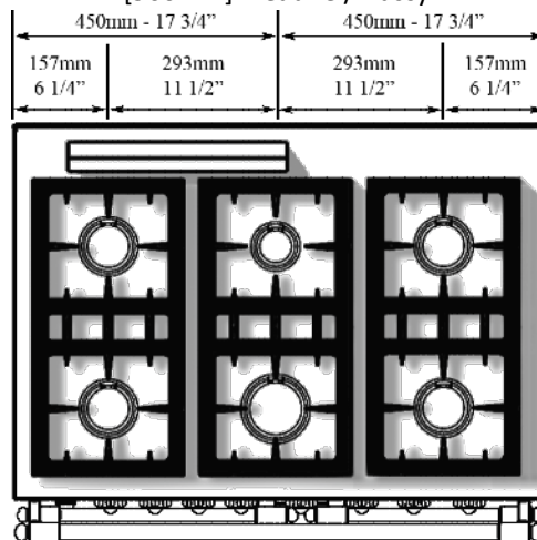
[900mm] Beaune / Bussy:
